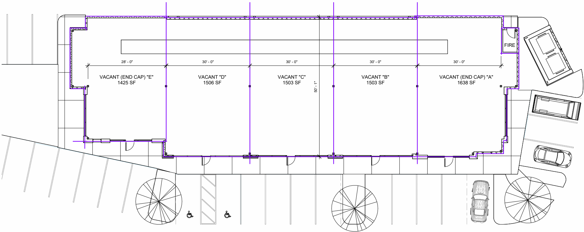
① LEASING FLOOR PLAN 1" = 10'-0"
